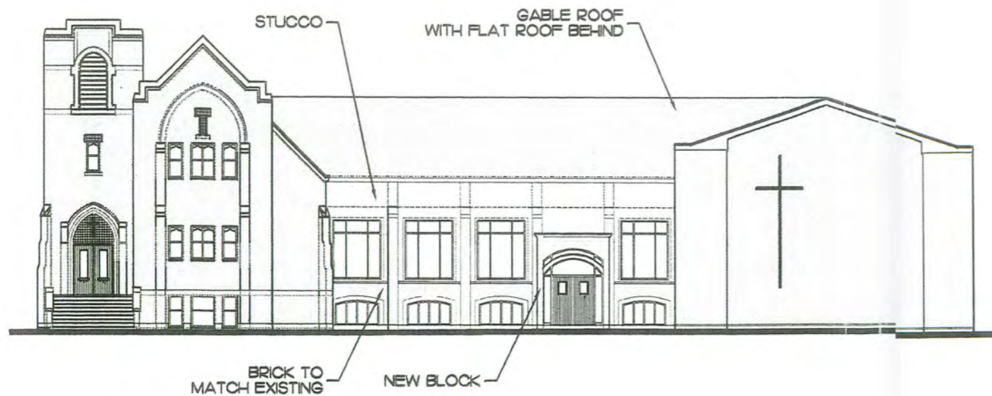
3 WEST ELEVATION 1/8" = 1'-0"
